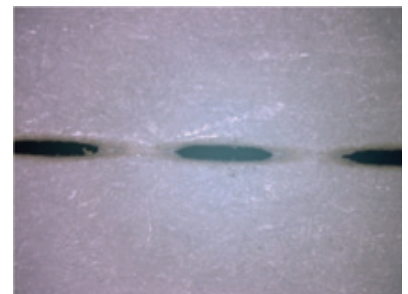
Long hole perforation of paper (80 g / m 2 ) Speed: 75 m / min
